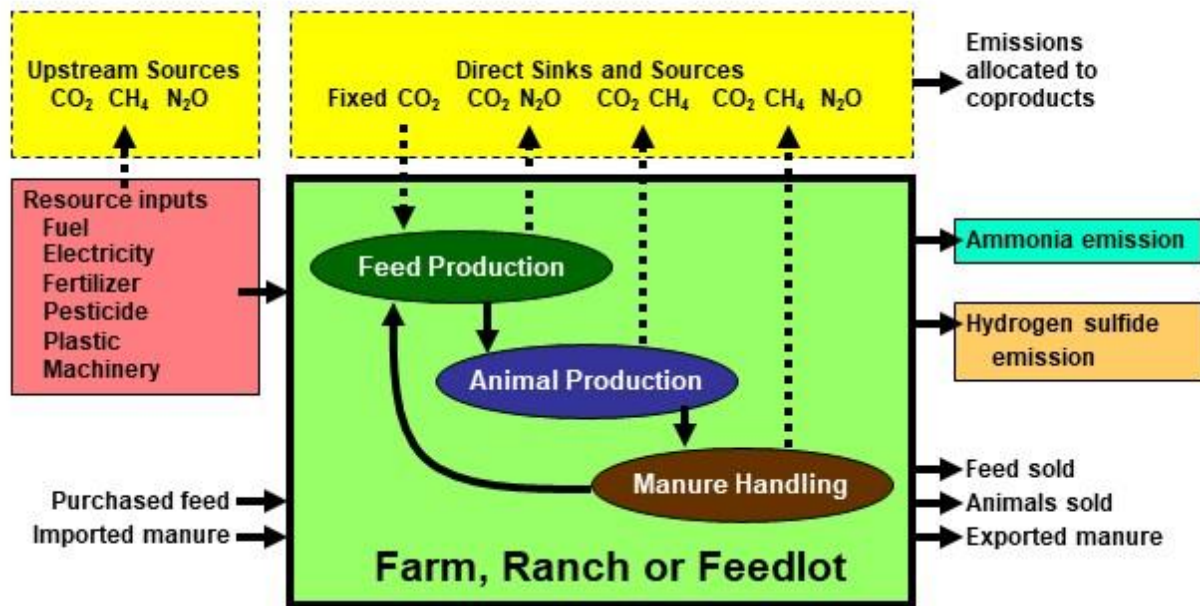
Figure 1.1. Important components, sources, and sinks considered in the emission of ammonia, hydrogen sulfide, greenhouse gases and the life cycle assessment determining the carbon footprint of cattle operations.
