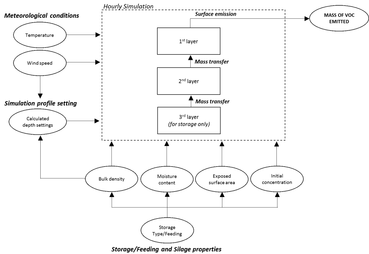
Figure 7.1. Diagram for the hourly simulation of VOC emissions from silage storage and feed lanes.
