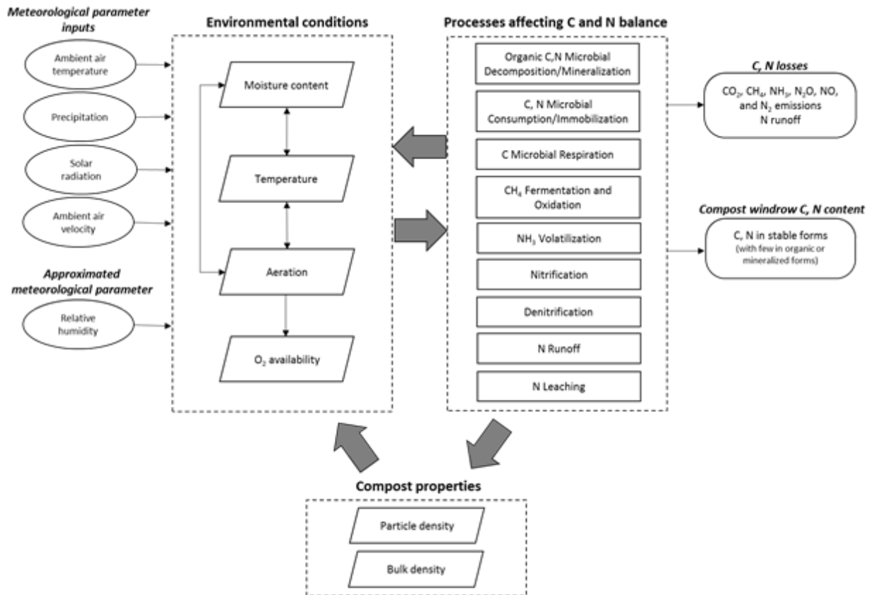
Figure 3.1. Model flow in the simulation of a compost windrow.
