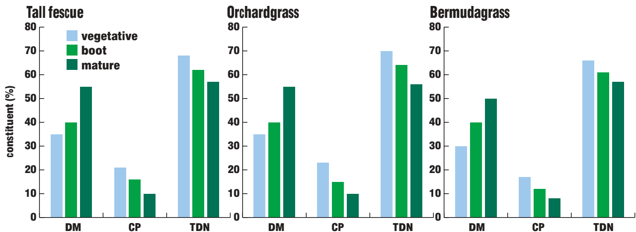
Figure 9. Forage quality dry matter (DM), crude protein (CP), and total digestible nutrients (TDN) percentages at varying growth stages.
